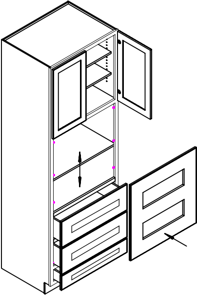
Assembly
